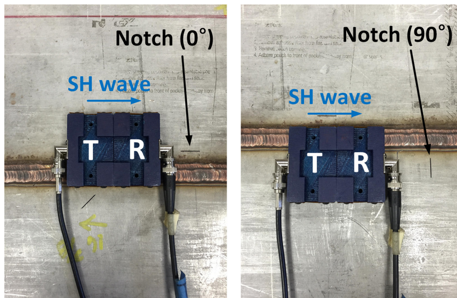
Fig. 10 EMAT arranged to detect notches oriented 0 deg (left) and 90 deg (right)
