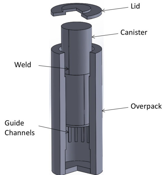
Holtec HI-STORM 100 System
