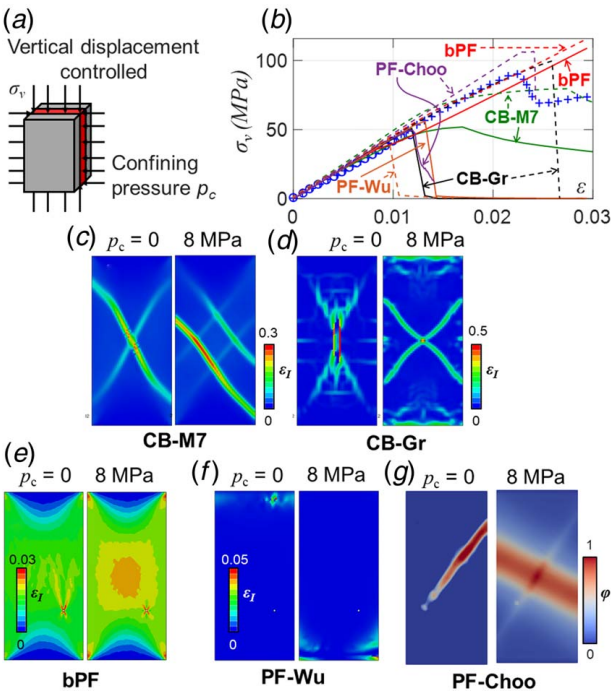
Fig. 11 Fracture of transversely confined sandstone slab under constant lateral confining pressure: (a) the loading configuration, (b–g) comparisons between the CB and PF predictions, including nominal stress–strain responses (b) and damage pattern (c–g)
