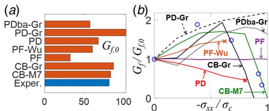
Fig. 21 (a) The deviations from the experimental fracture energy of CB, PF, and PD models. (b) Gap test results showing the relative change of measured concrete fracture energy G_f versus crack-parallel compression \sigma_{xx} , normalized by uniaxial compression strength \sigma_c , and comparisons to CB, PF, and PD models.
