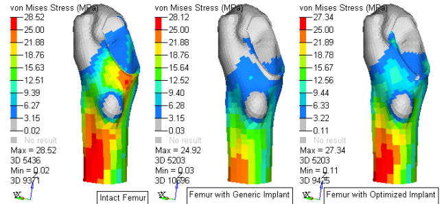
Figure 12: Stress Shielding is Reduced with Optimized Implant under Stairs Up Load (LC4)
