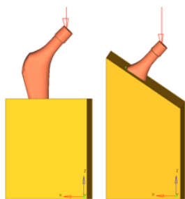
Figure 7: ISO Stem (left) and ISO Neck (right) Tests
