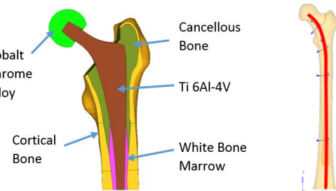
Figure 4: Material assignment in FE Model
