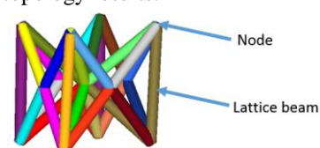
Figure 9: Face and Body Centered Cubic with Vertical Struts Unit Cell
